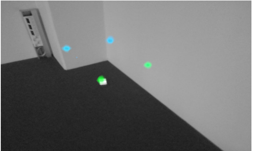
An example of one actual sound source and three reflections shown by the NL Camera in multi-source mode. The actual sound source lies on the floor, while there are three reflections shown on the walls. When the camera is moved around, the location of the actual sound source remains the same, while the reflections move around on the walls, and are not seen from all angles.
